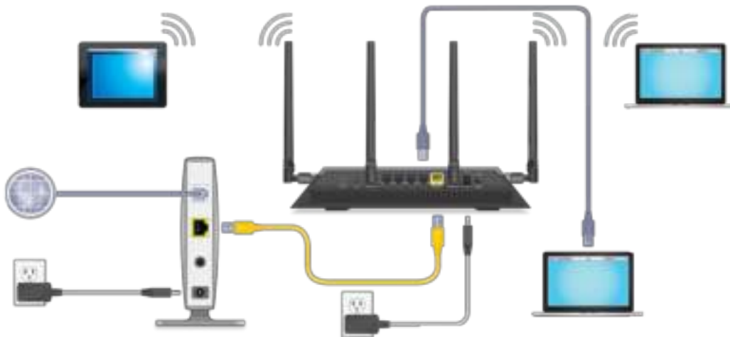
Figure 6. Router cabling
