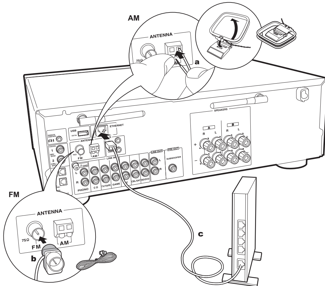
a AM indoor antenna, b FM indoor antenna, c Ethernet Cable
