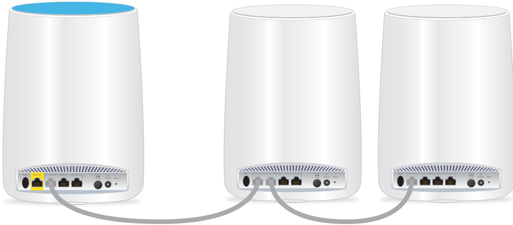
Figure 2. Satellite 1 connected to router and satellite 2 connected to satellite 1
