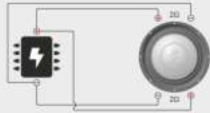
Serial wiring → 4 Ohms
