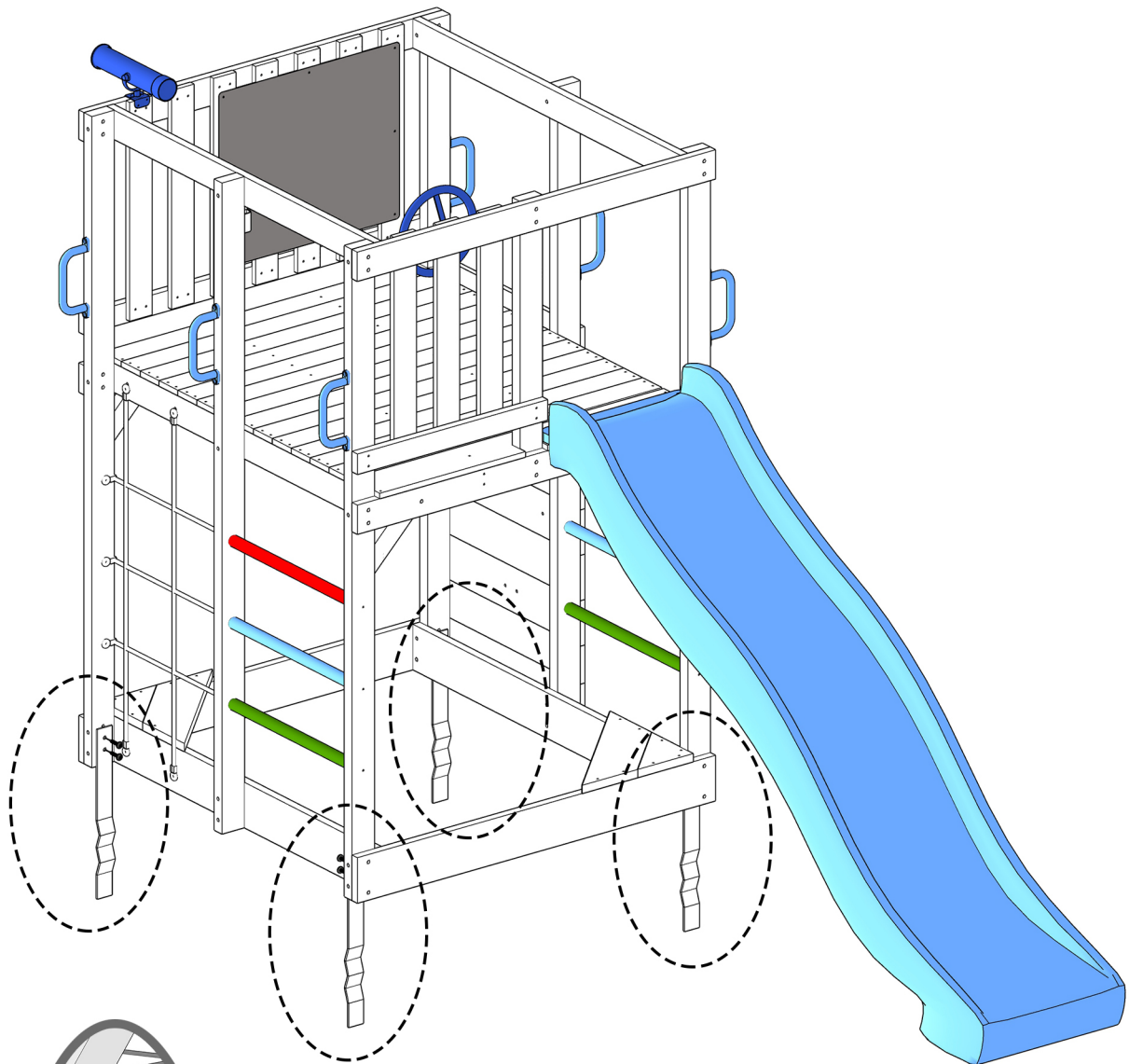
Anchors-139070
