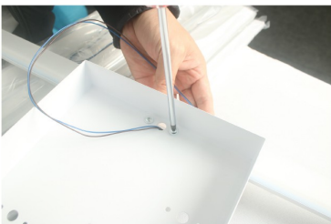
4, turn around and fasten the petal with screws. Assemble all the petals as the same way
