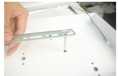
6, put down the hanger, make sure the screws can go through the two holes at the plate, then fasten the nuts to lock the positions of each screw
