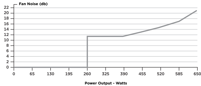
Corsair RM650x power supply fan noise curve
