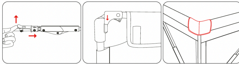
R1-R4 Lock-systeem
