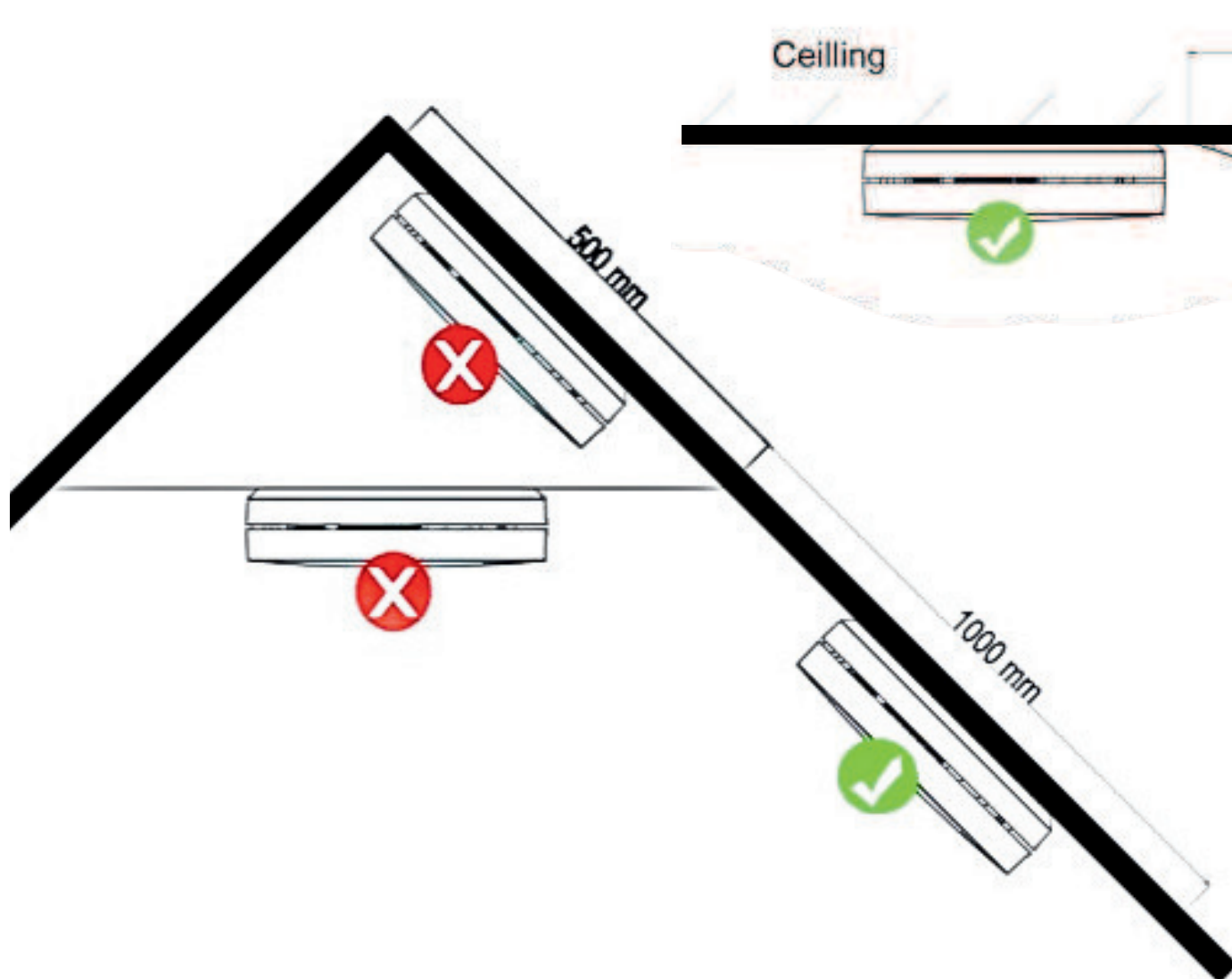
Figure 4: Recommended mounting locations
