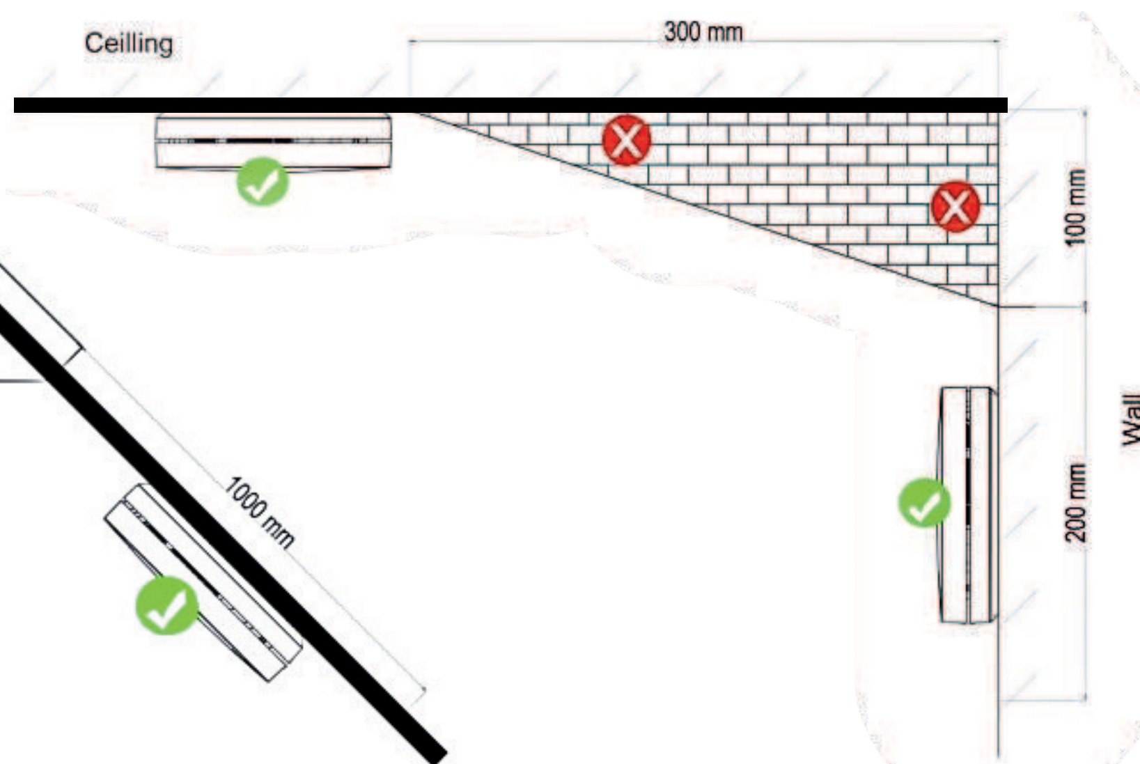
Figure 5: Recommended mounting locations
