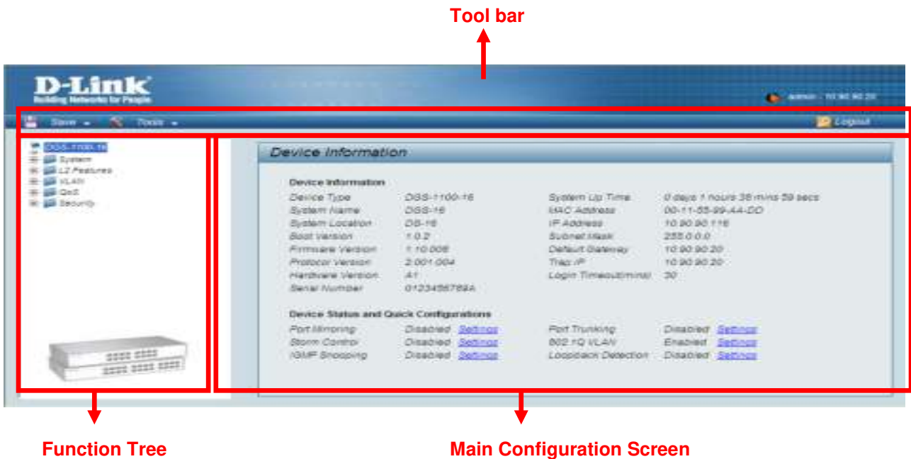
Figure 33 – Web-based Management
