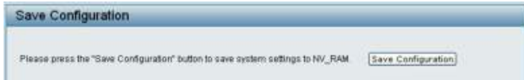
Figure 35– Save Configuration
