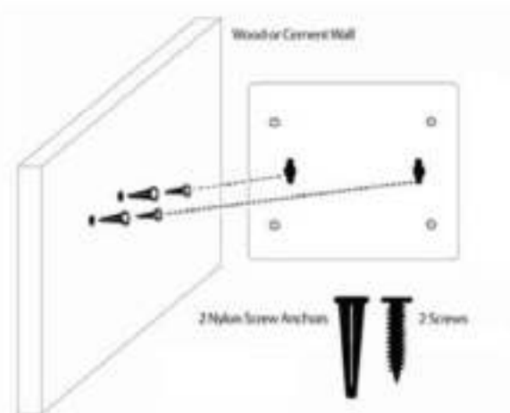
Figure 14 –Wall mount installation
