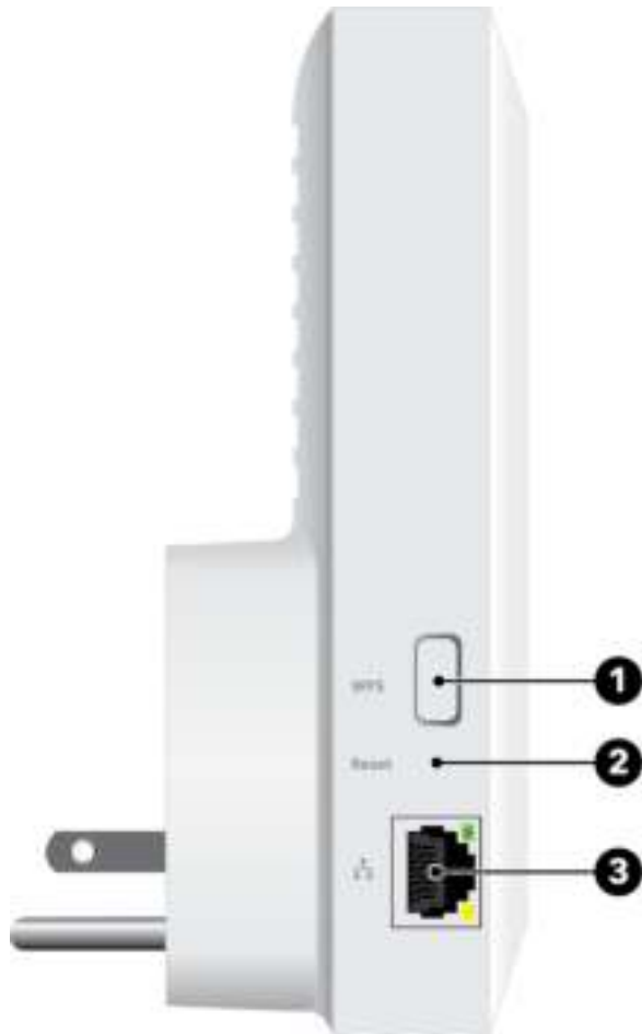
Figure 3. Back panel
