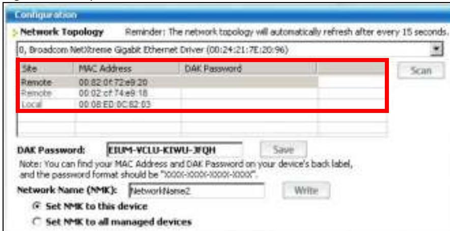
Figure 35 Adapters on a New Powerline Network
