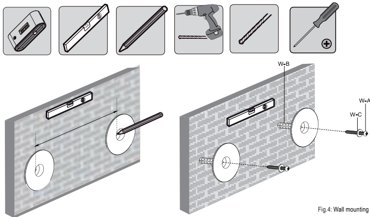
Fig.4: Wall mounting
