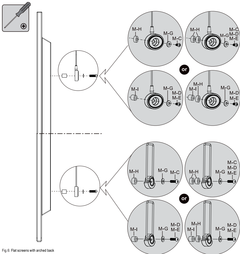
Fig 6: Flat screens with arched back
