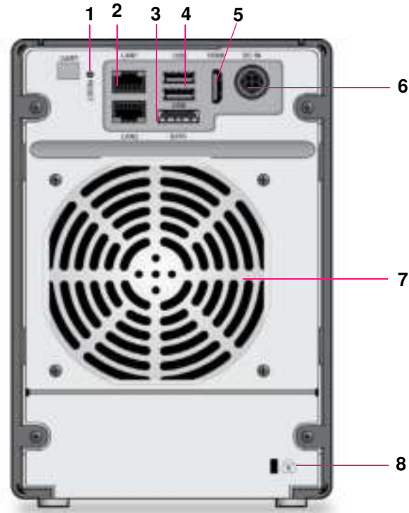
Figure 26. ReadyNAS 314 rear panel
