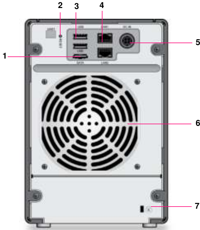
Figure 13. ReadyNAS 204 rear panel
