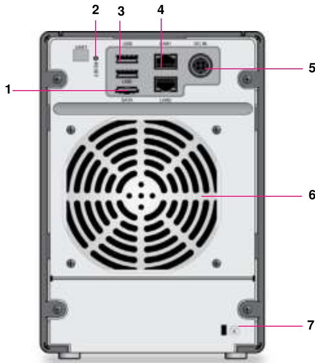
Figure 6. ReadyNAS 104 rear panel
