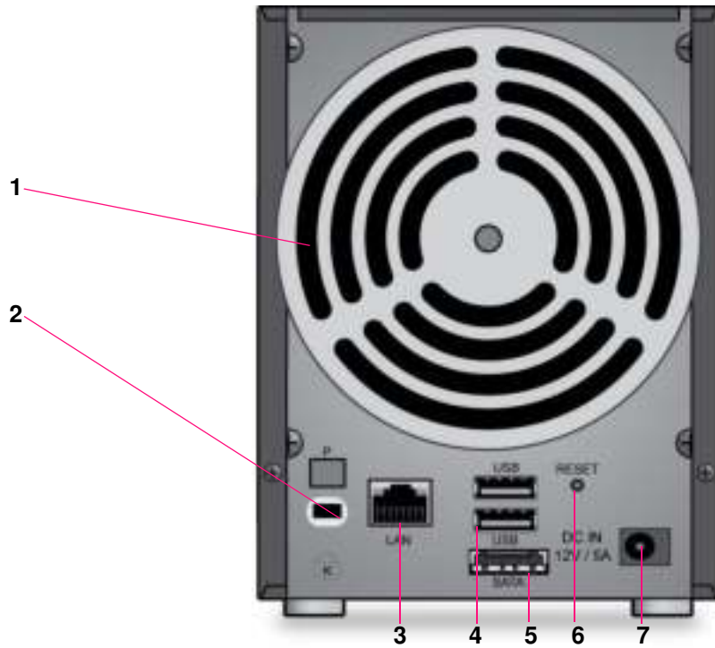
Figure 3. ReadyNAS 102 rear panel
