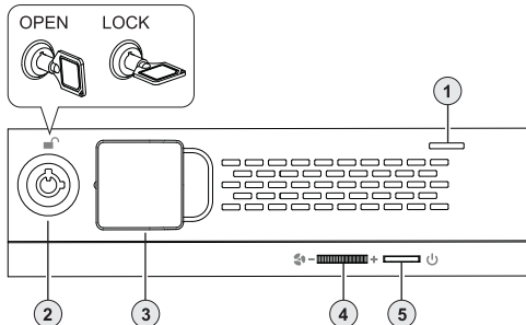
Front Panel
