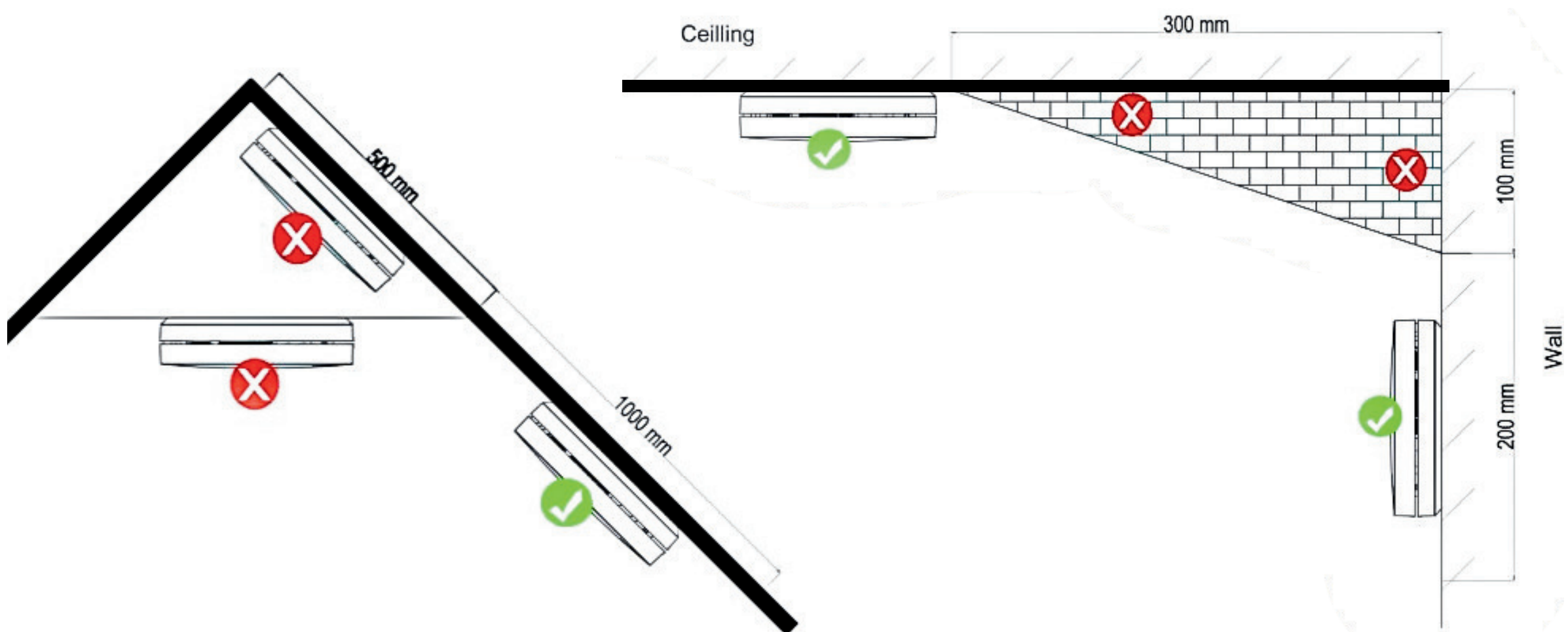
Figure 4: Recommended mounting locations
