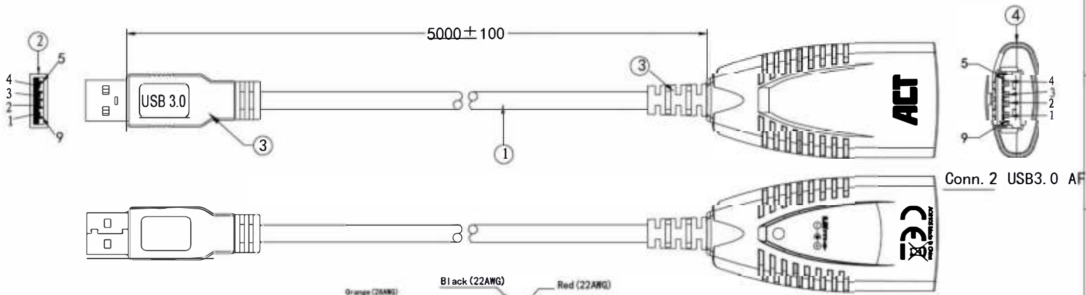
Conn. 1 USB3.0 A Type Male
