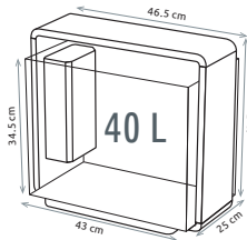
Home 45 High Power LED lighting: 12 V/12 W Aqua Flow 100 pump: 3.5 W, 50 - 200 l/h
