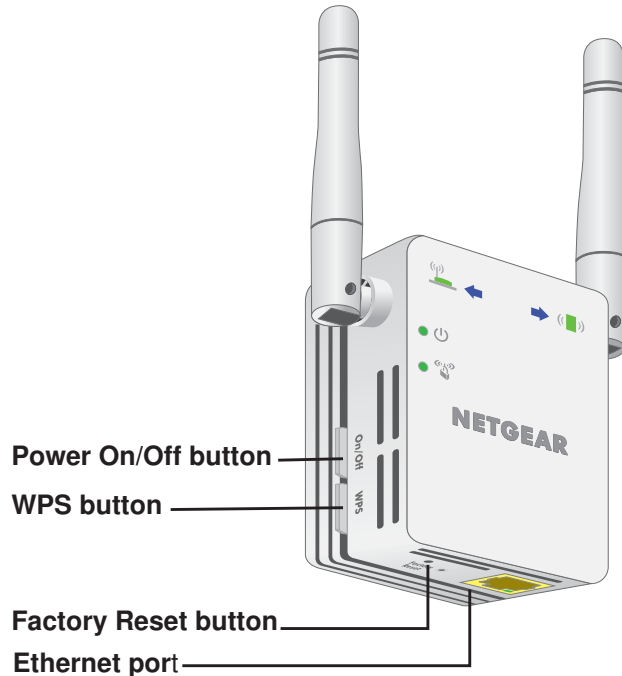
Figure 2. Extender side and bottom panels
