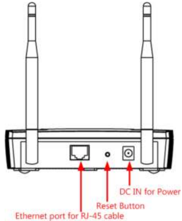
Rear Panel
