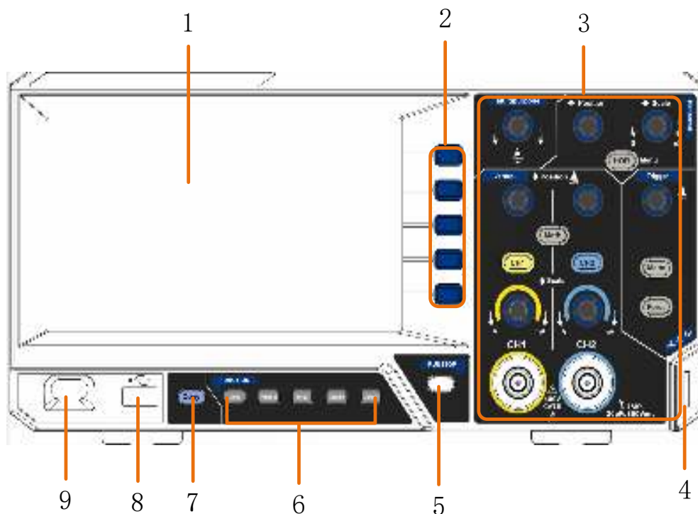
Figure 3-1 Front panel
