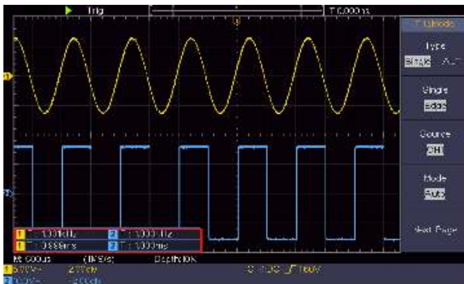
Figure 4-13 Automatic measurement
