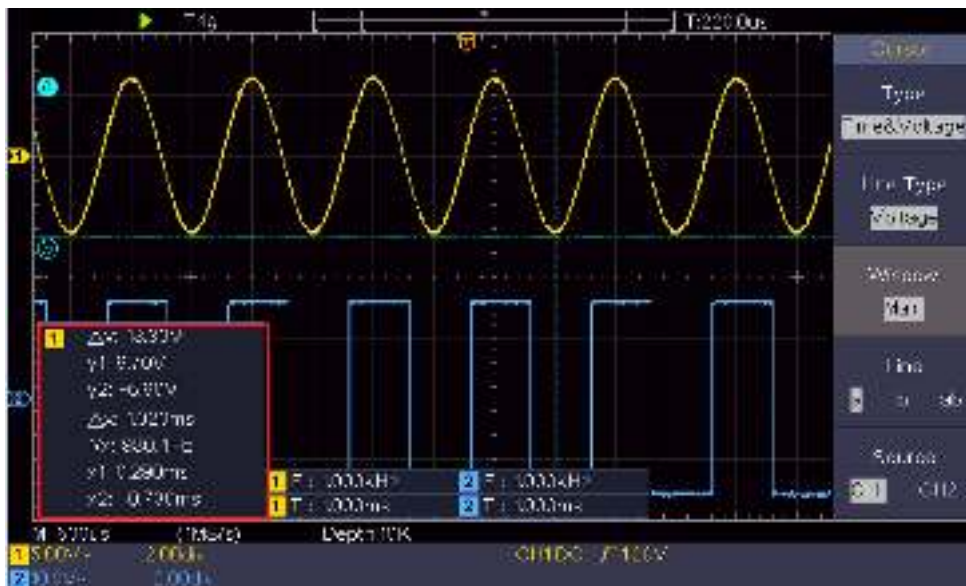
Figure 4-16 Time&Voltage Cursor Measurement
