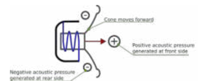
Figure 2 - Generic driver
