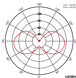
DROP 7,5W
