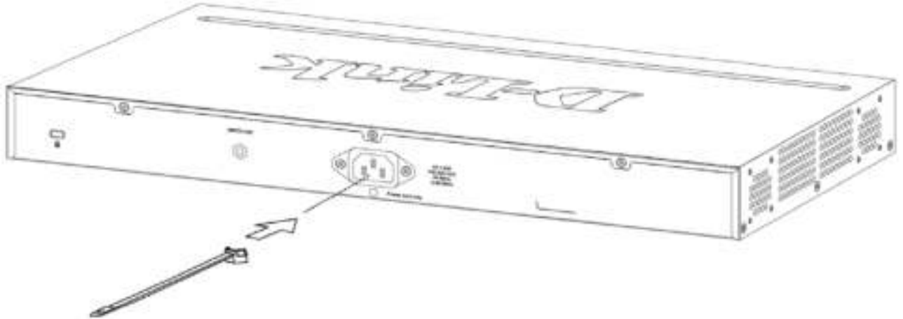
Figure 2-5 Insert Tie Wrap to the Switch
