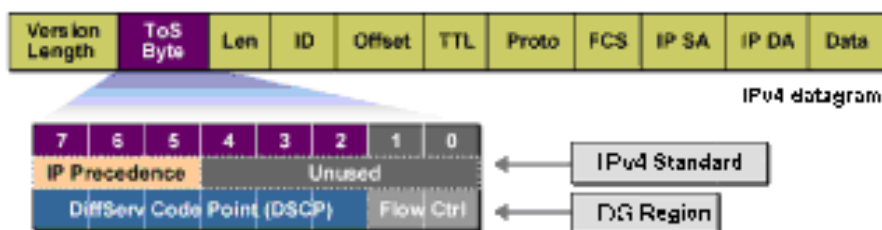
Figure 8-4 IP datagram
