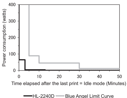
Power consumption and default times of HL-2240D during time elapsed after the last print
