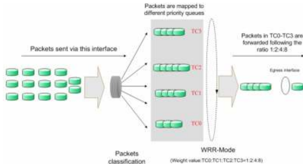
Figure 9-5 WRR-Mode
