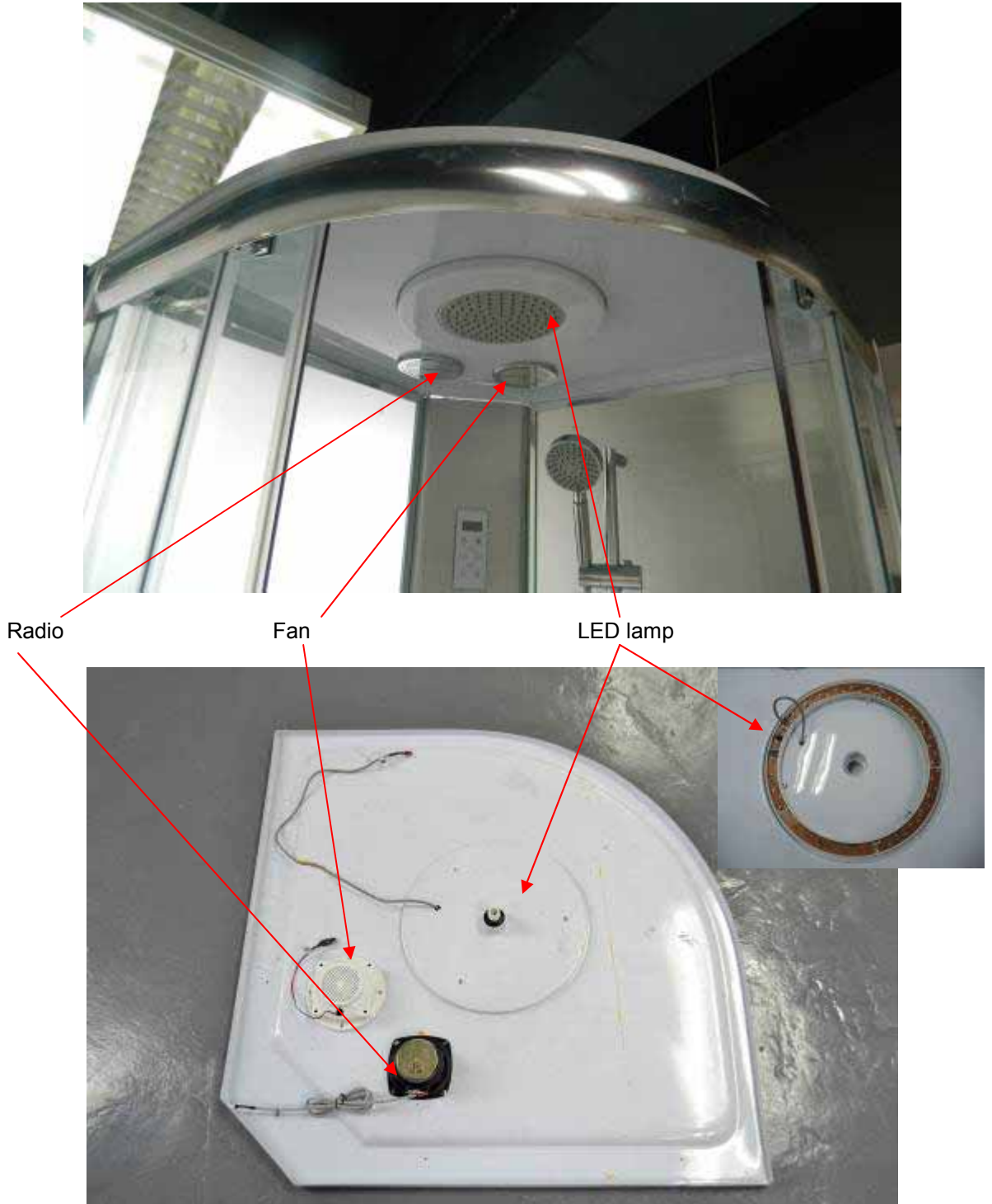
Up enclosure view
