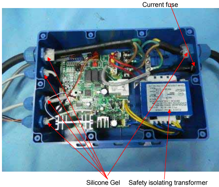
Power box internal view
