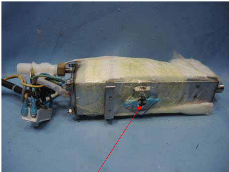
Self-resetting thermal cut-out for steam generator (connected to SELV)
