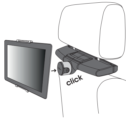
3 Flex Mount
