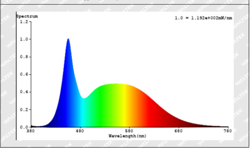
Model: LED module for 360bbyy-xx(6500K)
