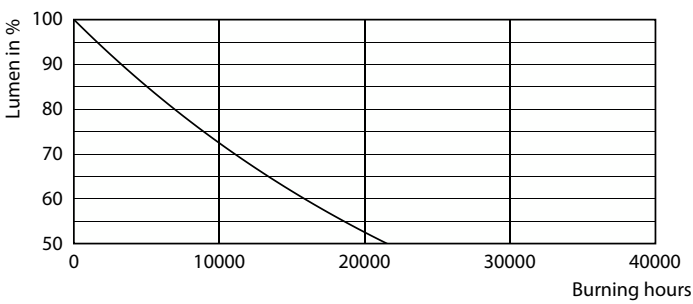
Lumen Maintenance Diagram - CorePro LEDbulb ND 8-60W A60 E27 865
