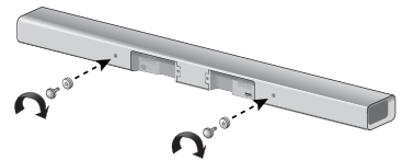
Wall Mounting the Soundbar
