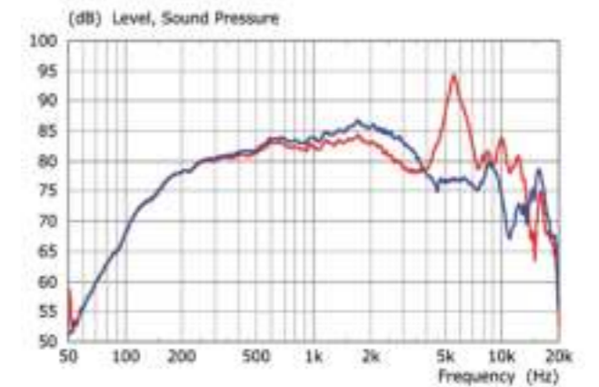
Figure 37 Effect of lossy interface on response of LF/MF driver
