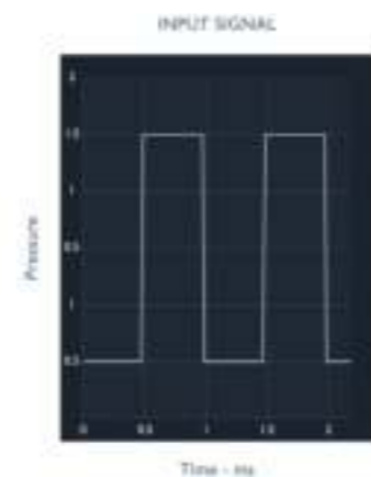
Figure 56 Input signal - 1kHz square wave
