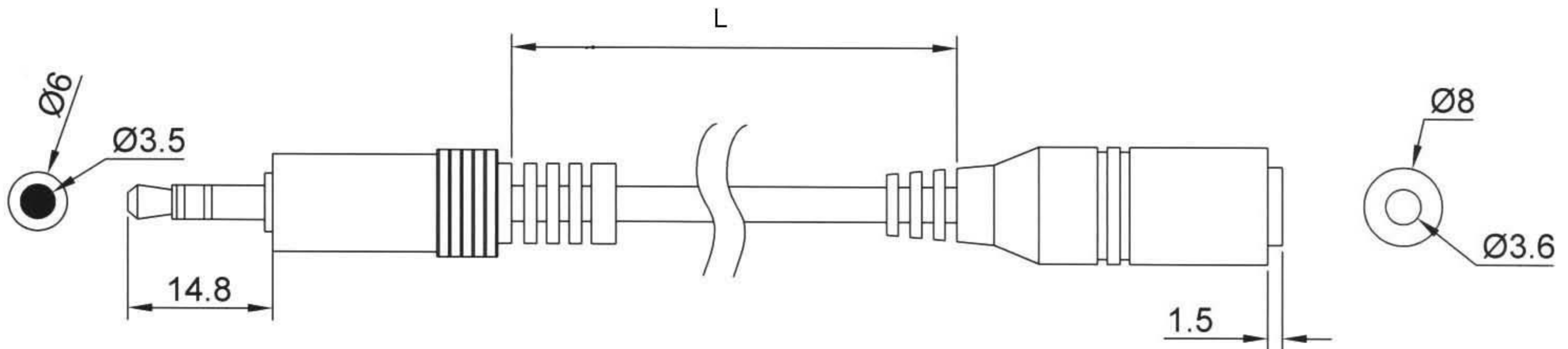
3.5 stereo plug
