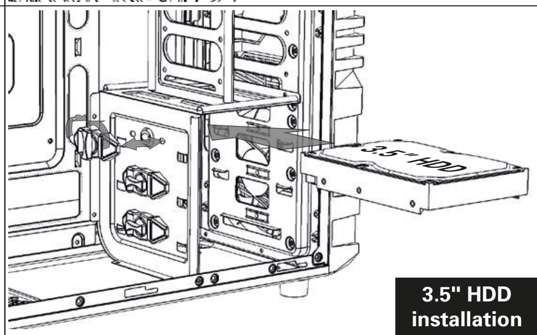
3.5" device installation
