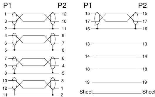
Wire method
