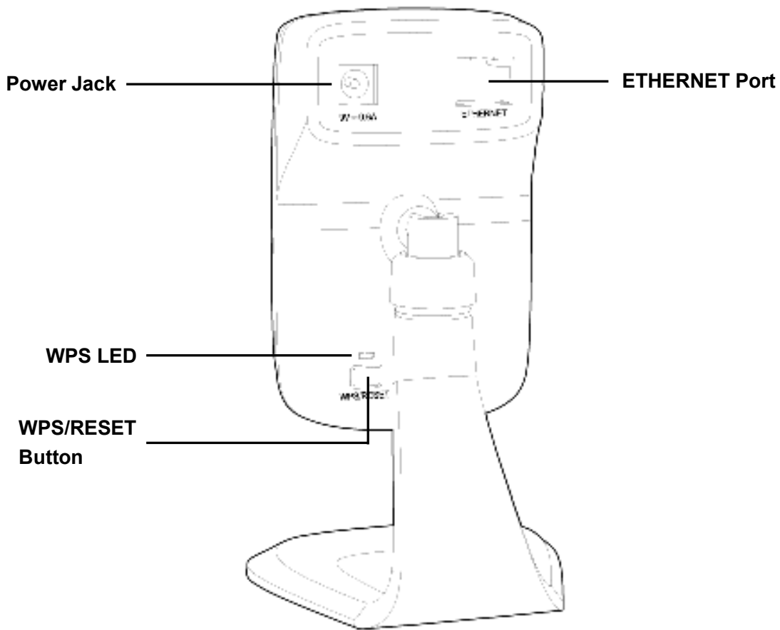
Figure 2-2 Rear Panel
