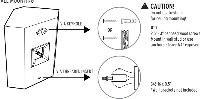
FIGURE 4 WALL MOUNTING
