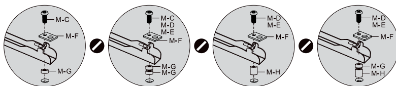
Fig. 10: Flat screens with arched back
