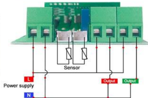
Connection 2: Same power supply for load
