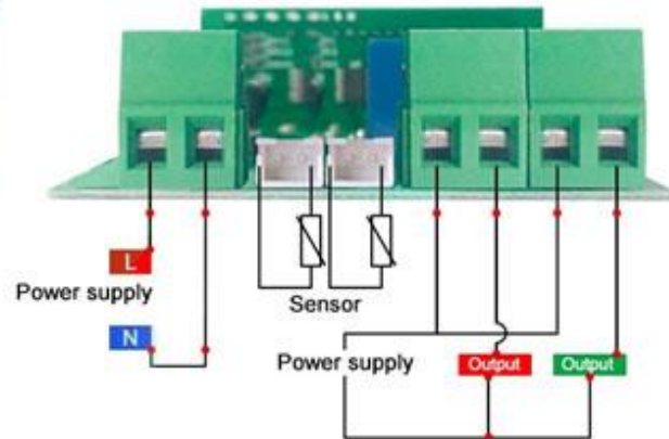
Connection 2: Same power supply for load
