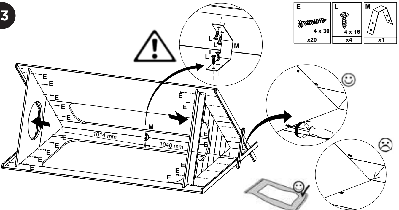
FRONT PANEL
