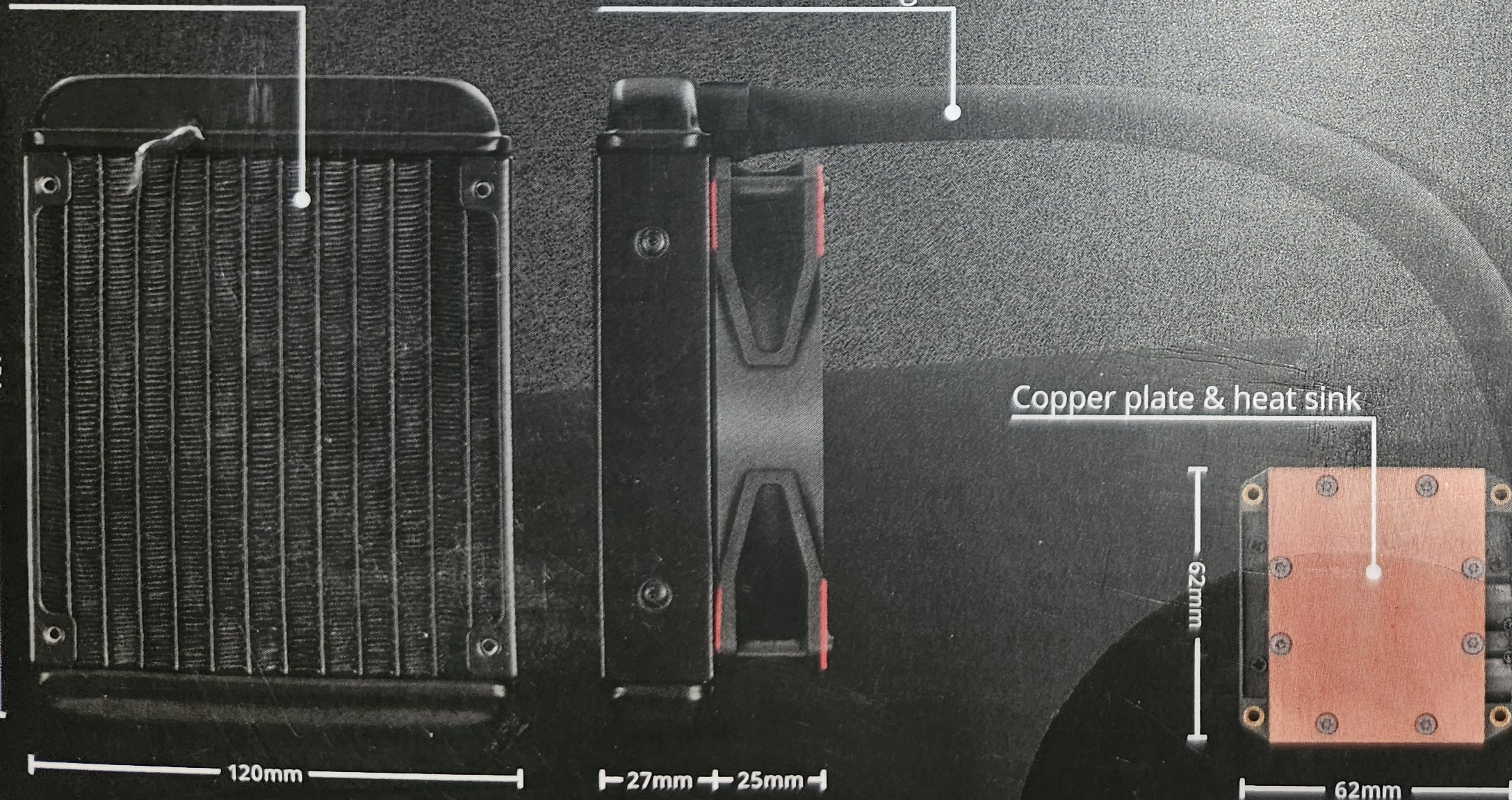
Aluminium radiator
