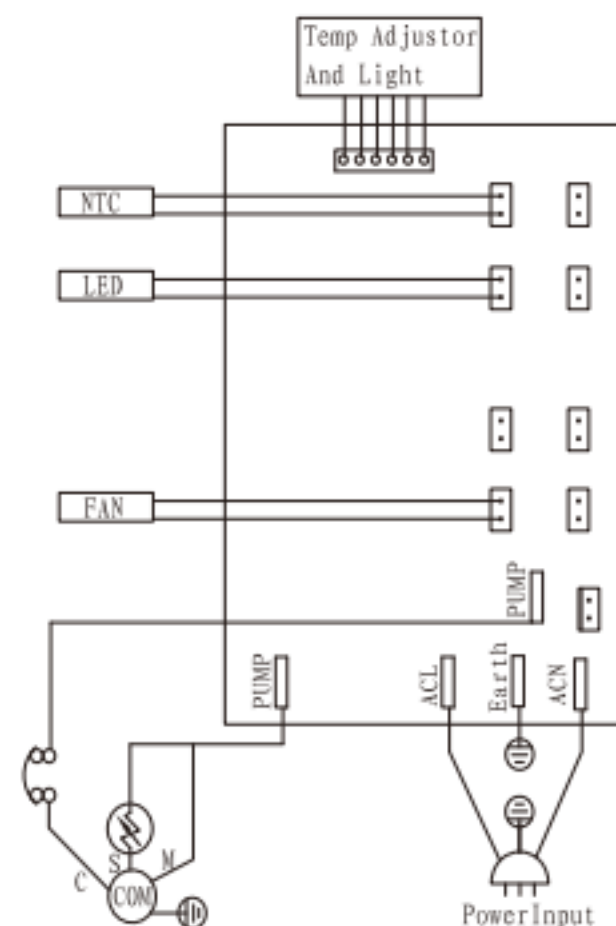
Electrocircuit Line Diagram
