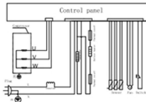
Diagram of Circuit Principles
