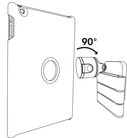
5 Flex Mount
