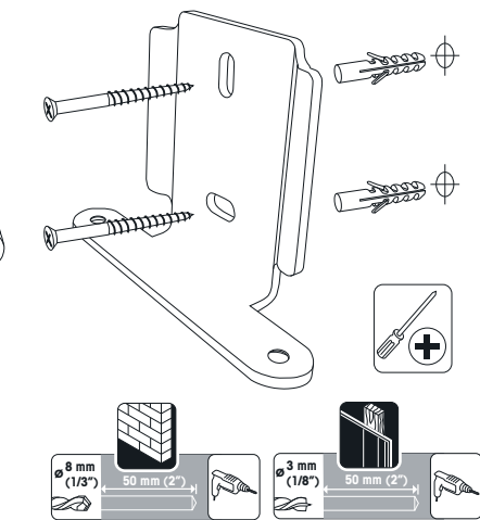
3 Flex Mount
