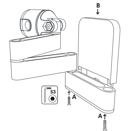
4 Flex Mount
