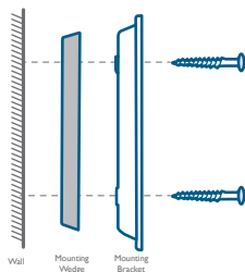
With 15° Mounting Wedge
