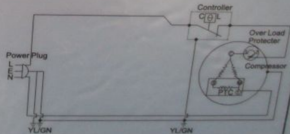
Circuit diagram
