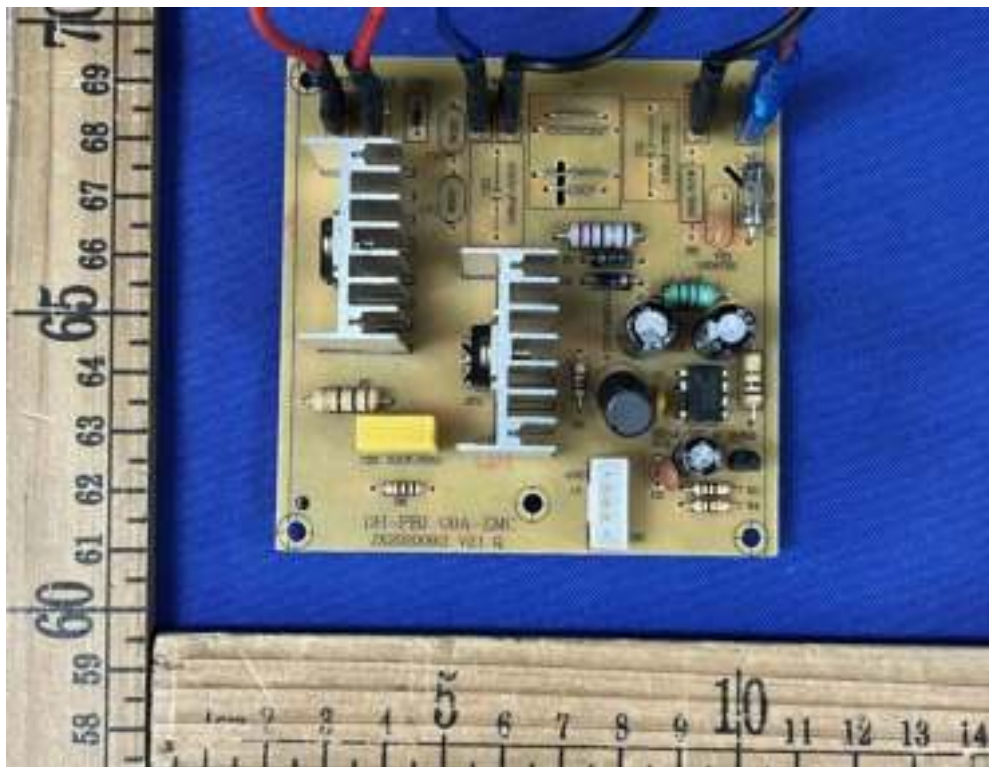
Figure 4 Front plate of PCB– model YJB32
