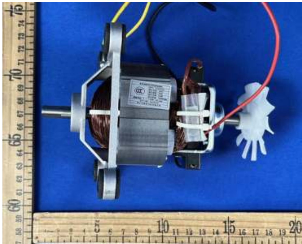
Figure 6 Motor– model YJB32
