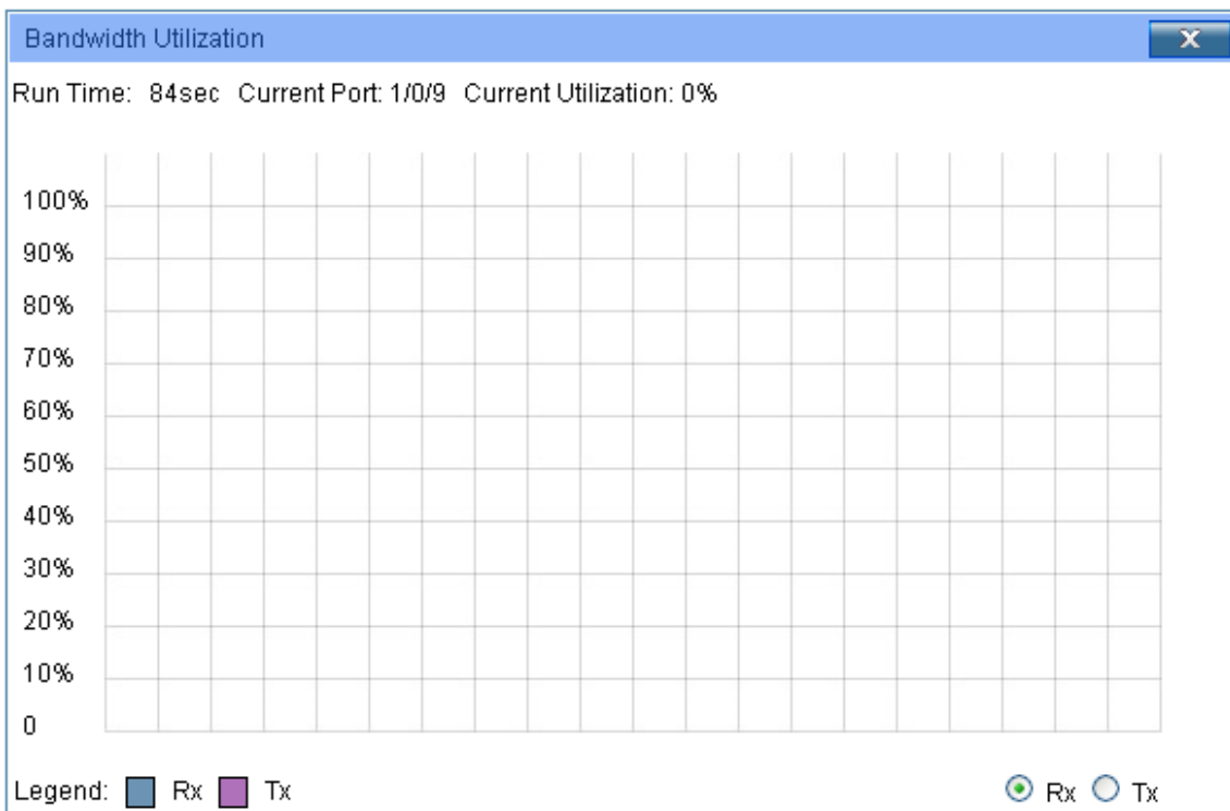
Figure 4-3 Bandwidth Utilization
