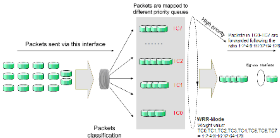
Figure 12-5 WRR-Mode
