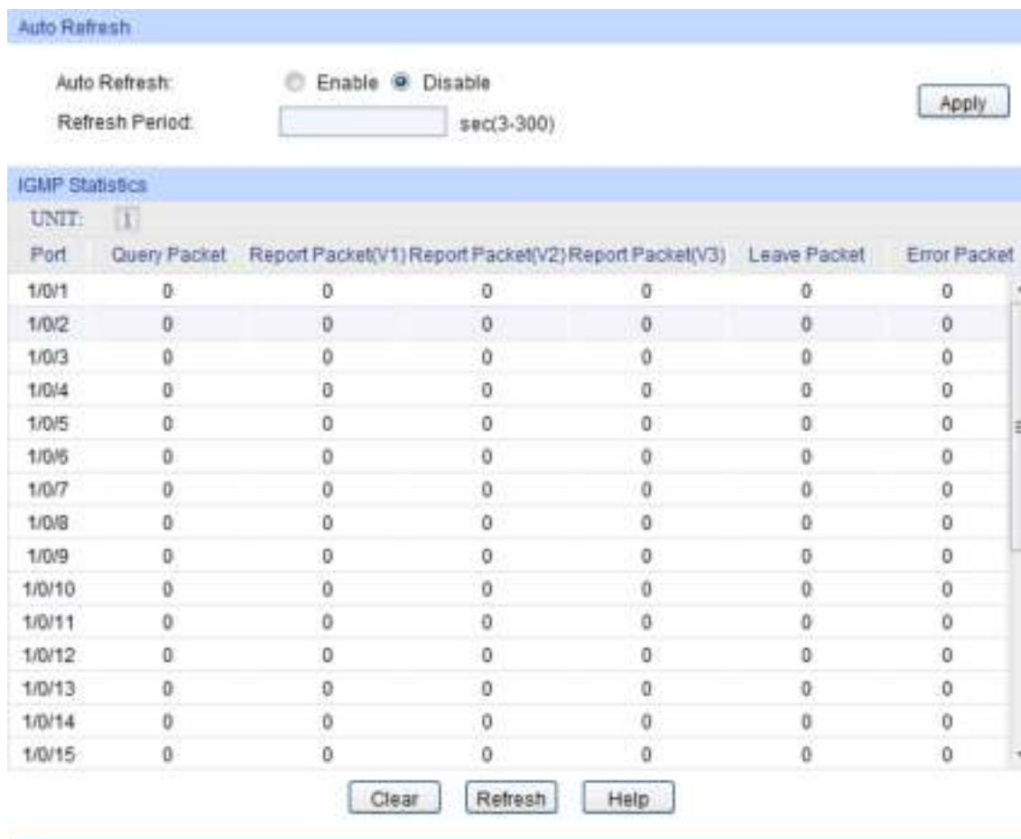
Figure 9-14 Packet Statistics
