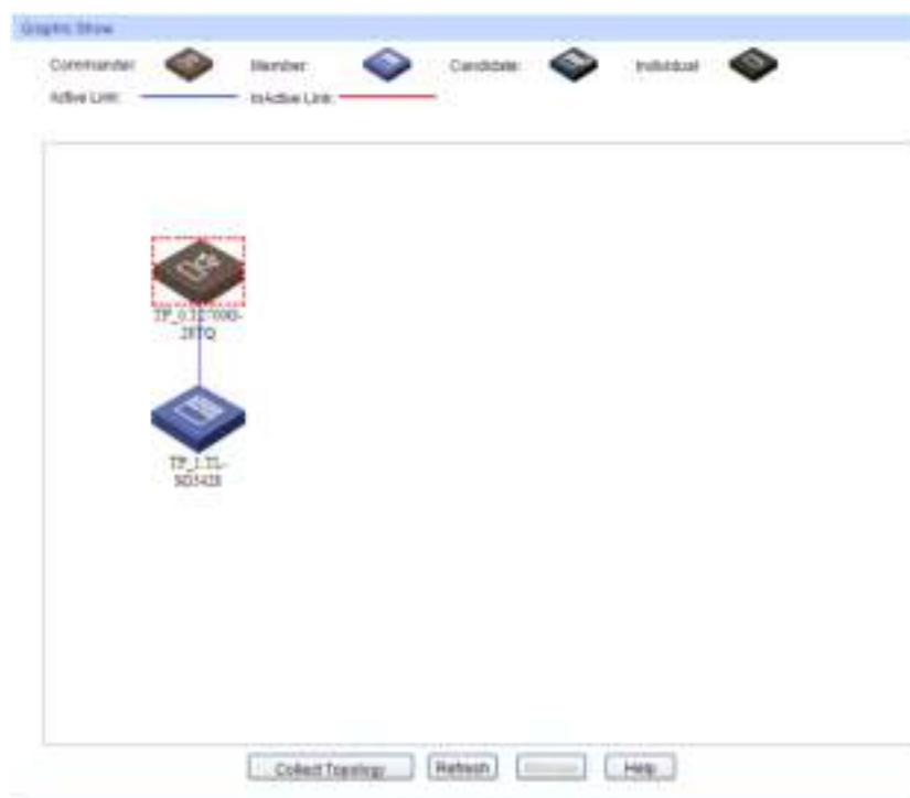
Figure17-18 Collect Topology
