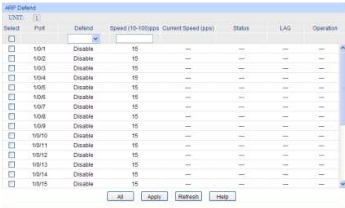
Figure 14-15 ARP Defend
