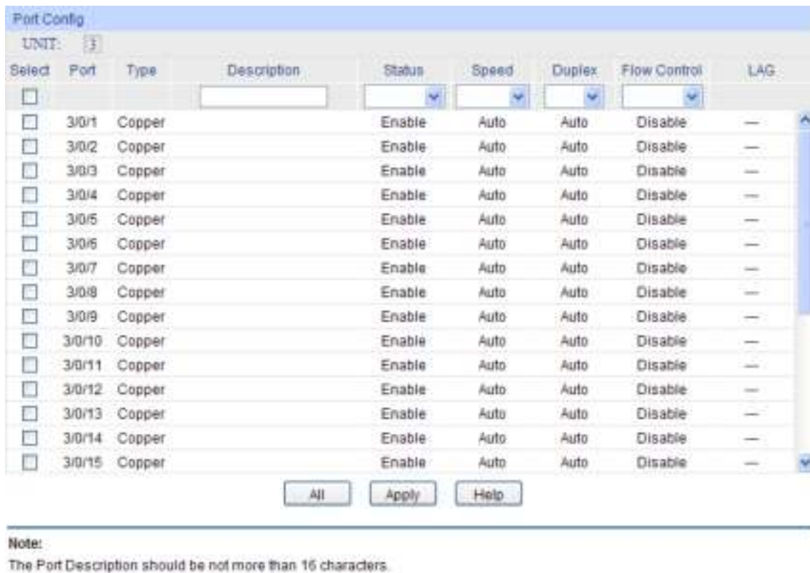
Figure 6-1 Port Config
