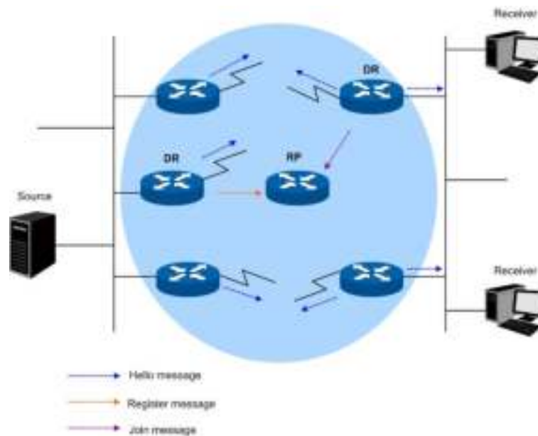
Figure 11-15 DR Elect
