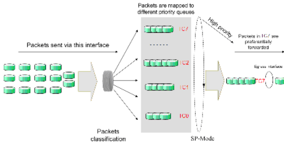
Figure 12-4 SP-Mode
