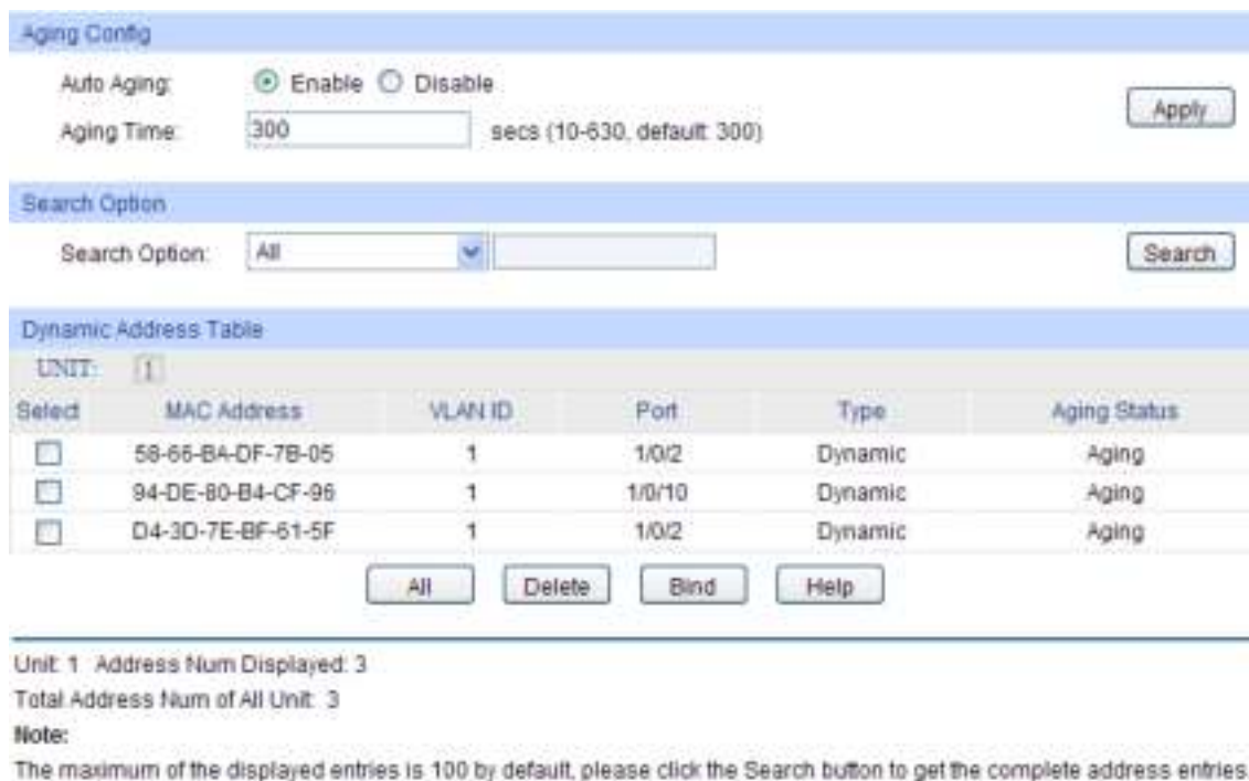
Figure 6-16 Dynamic Address
