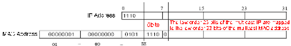
Figure 9-2 Mapping relationship between multicast IP address and multicast MAC address
