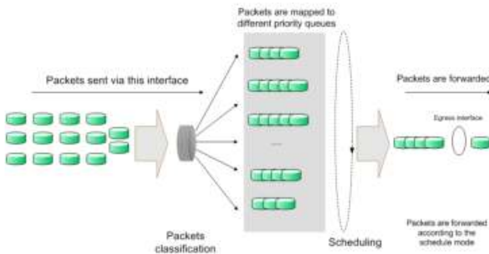
Figure 12-1 QoS function
