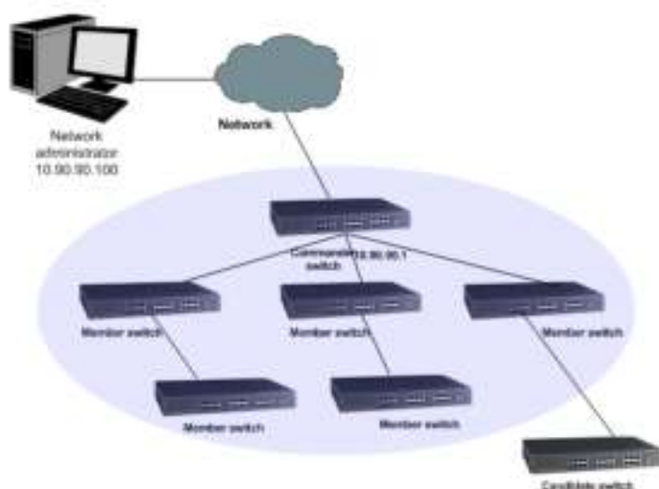
Figure17-1 Cluster topology
