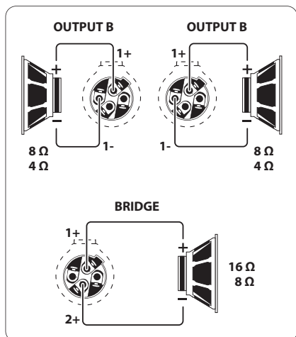
Fig. 4.7: Pin assignment
