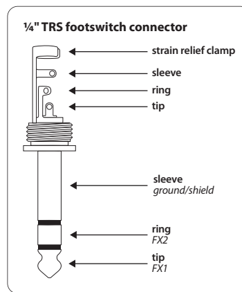
Fig. 4.4: 1/4" mono plug for footswitch
