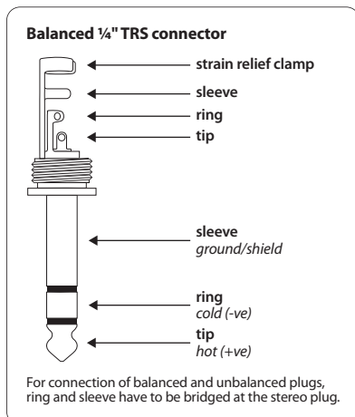
Fig. 4.2: 1/4" TRS connector
