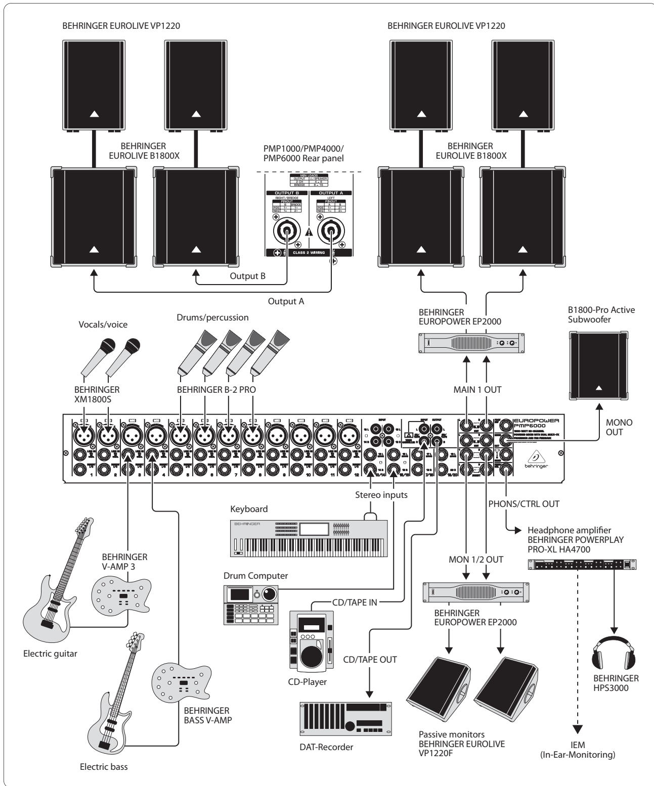
Fig. 5.5: Expanded set-up
